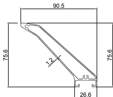
KU-539A 0.989KG/M
