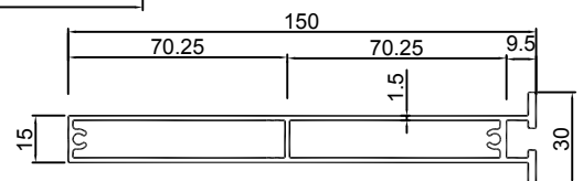
KU-429 1.587KG/M
